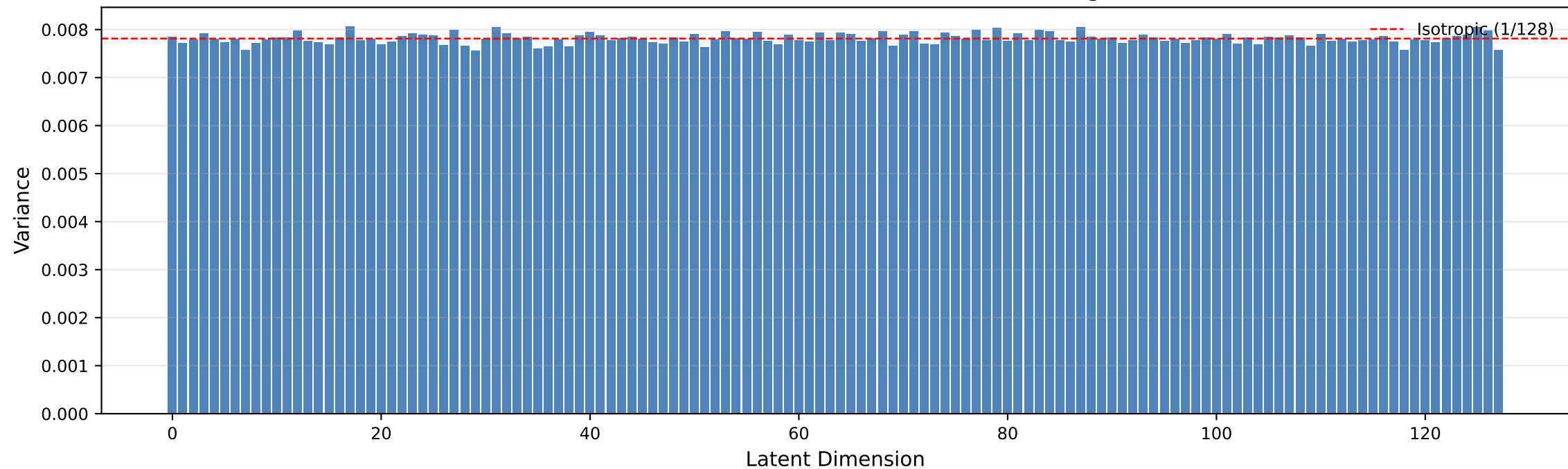
Per-Dimension Variance of Node2Vec Embeddings
