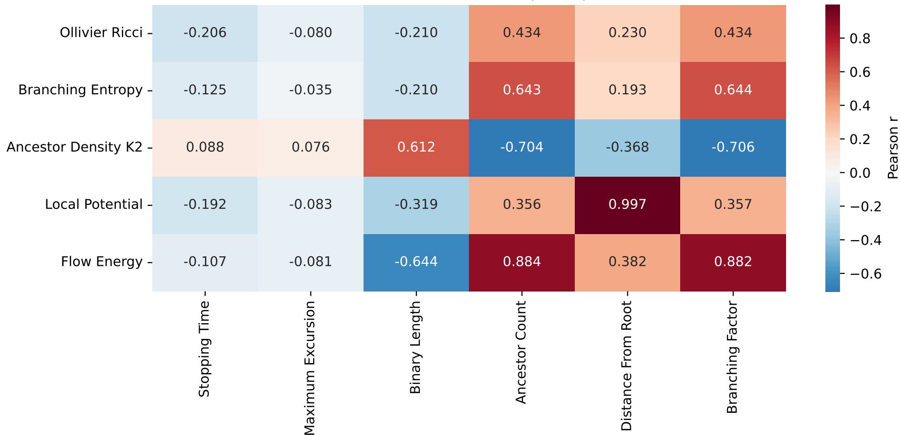
Geometric Quantities vs Graph Properties
