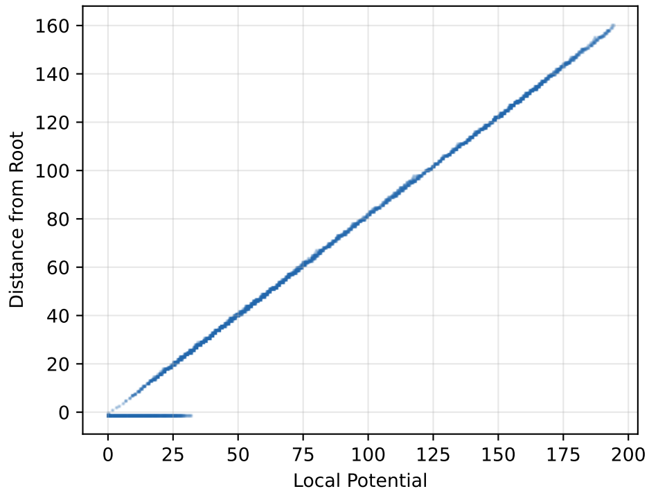
Local Potential vs Distance (r=0.9974)
