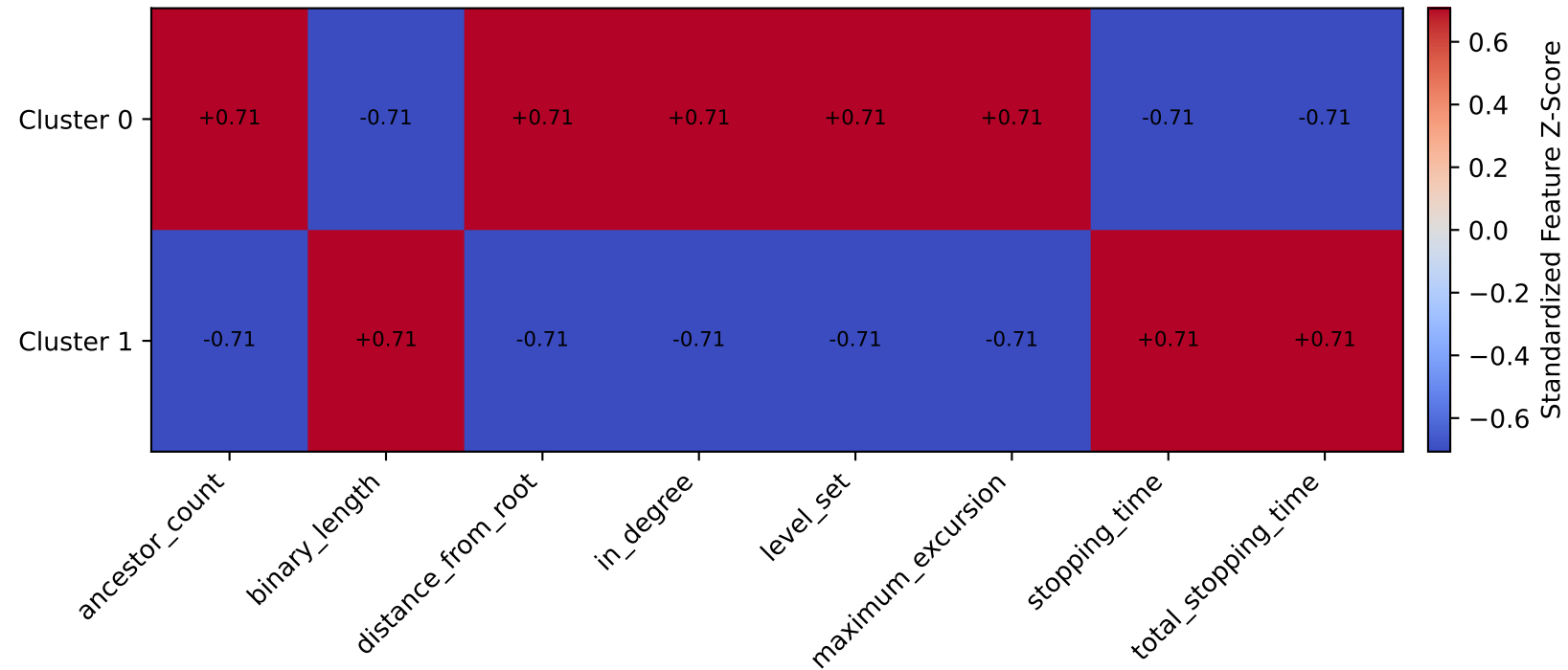
Standardized Collatz Property Profiles (HDBSCAN mcs=30)
