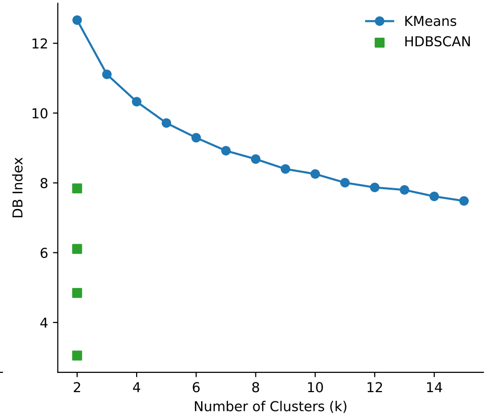
Davies-Bouldin Score (Lower is better)
