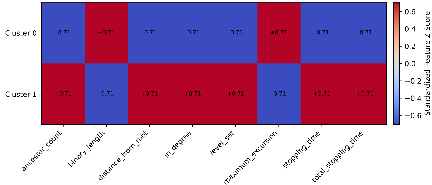
Standardized Collatz Property Profiles (KMeans k=2)
