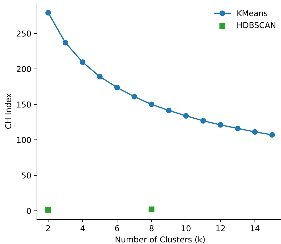
Calinski-Harabasz Score (Higher is better)
