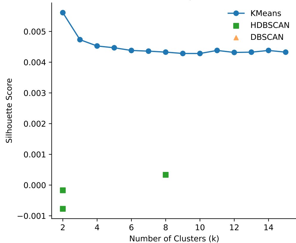
Silhouette Score (Higher is better)
