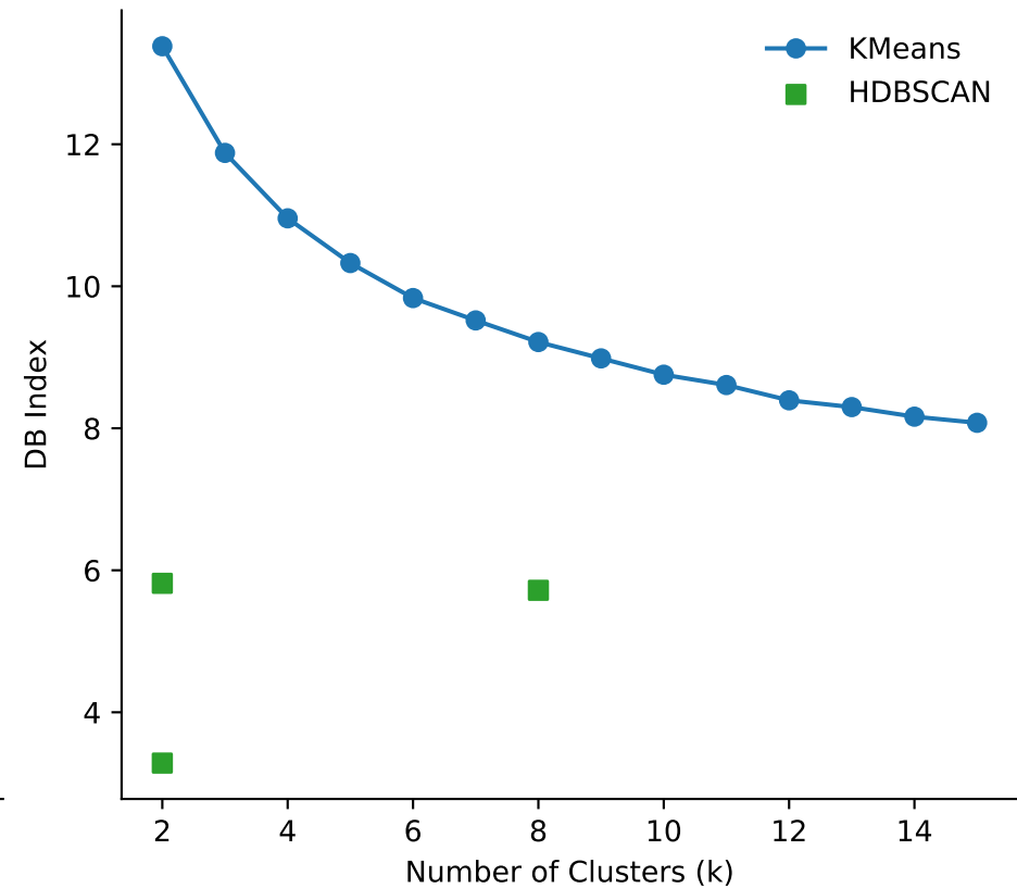
Davies-Bouldin Score (Lower is better)
