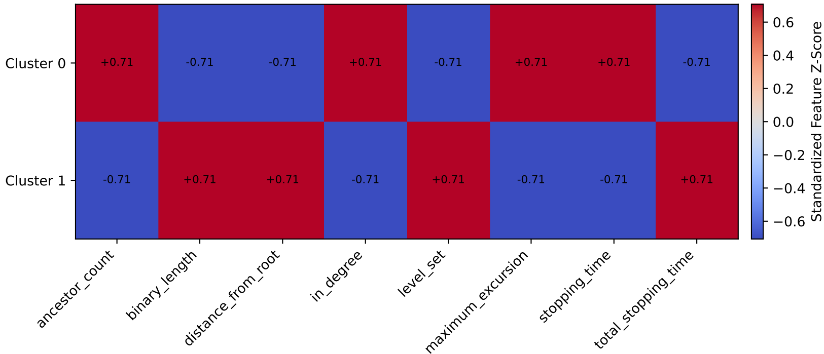
Standardized Collatz Property Profiles (KMeans k=2)
