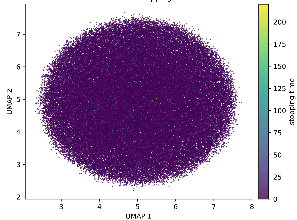
N=100000 — stopping time
