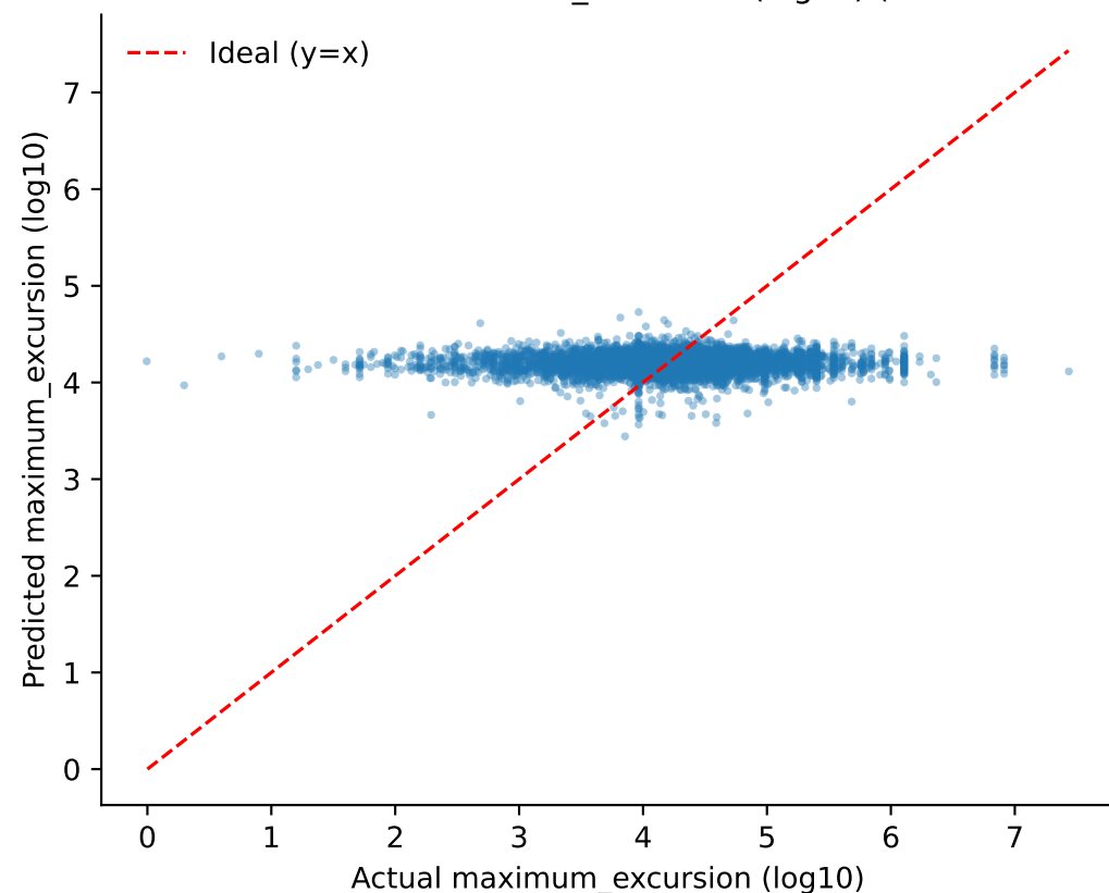
Actual vs Predicted: level_set (RandomForest)
