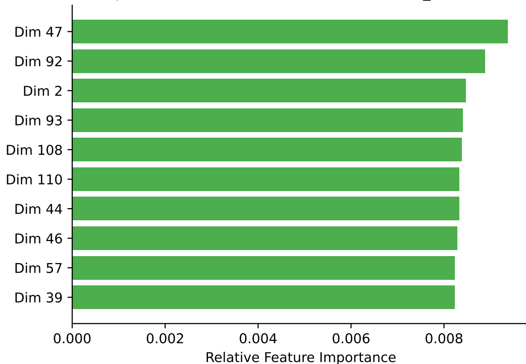
Top 10 Node2Vec Dimensions for level_set
