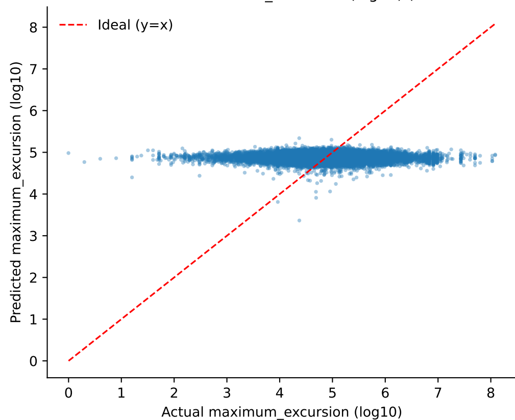
Actual vs Predicted: level_set (RandomForest)
