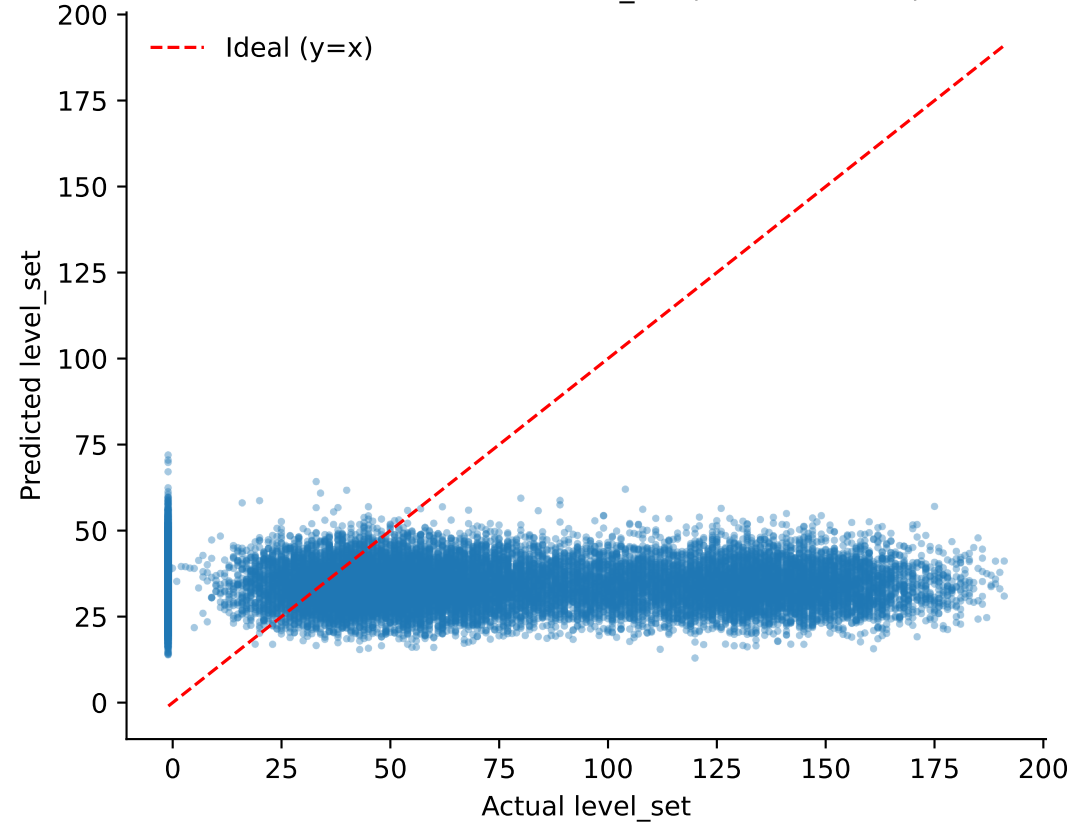
Actual vs Predicted: level_set (RandomForest)
