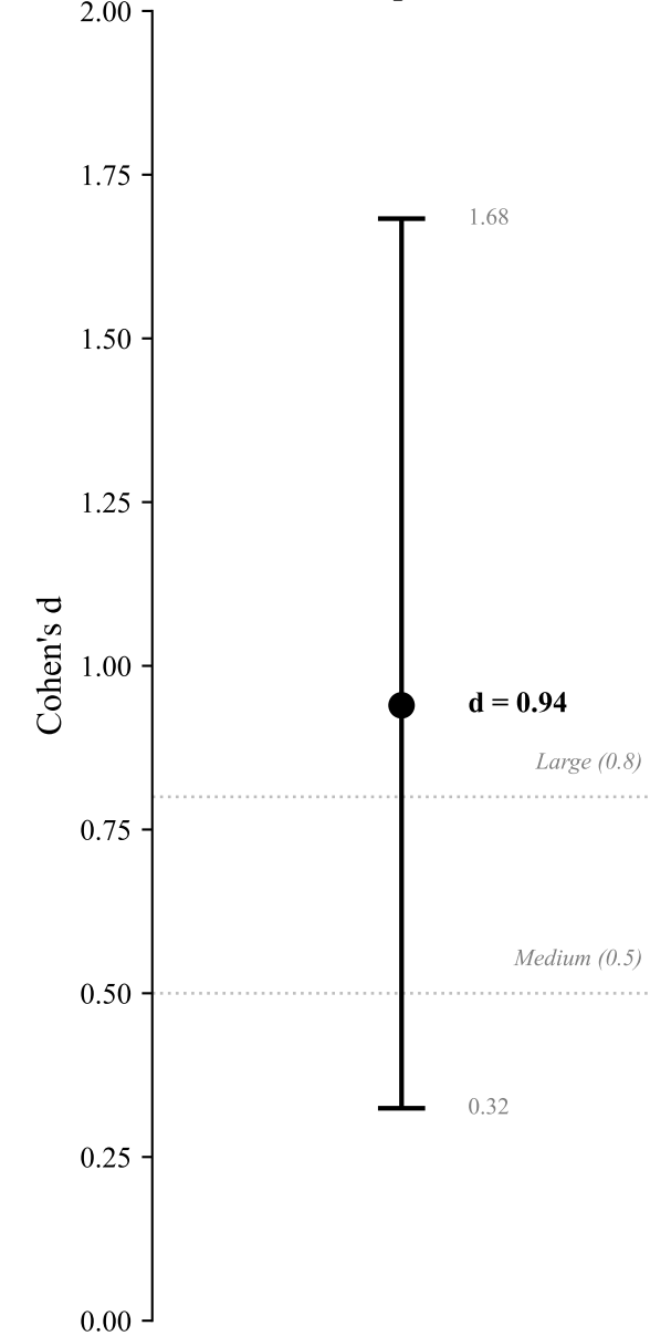
Bootstrap 95% CI
