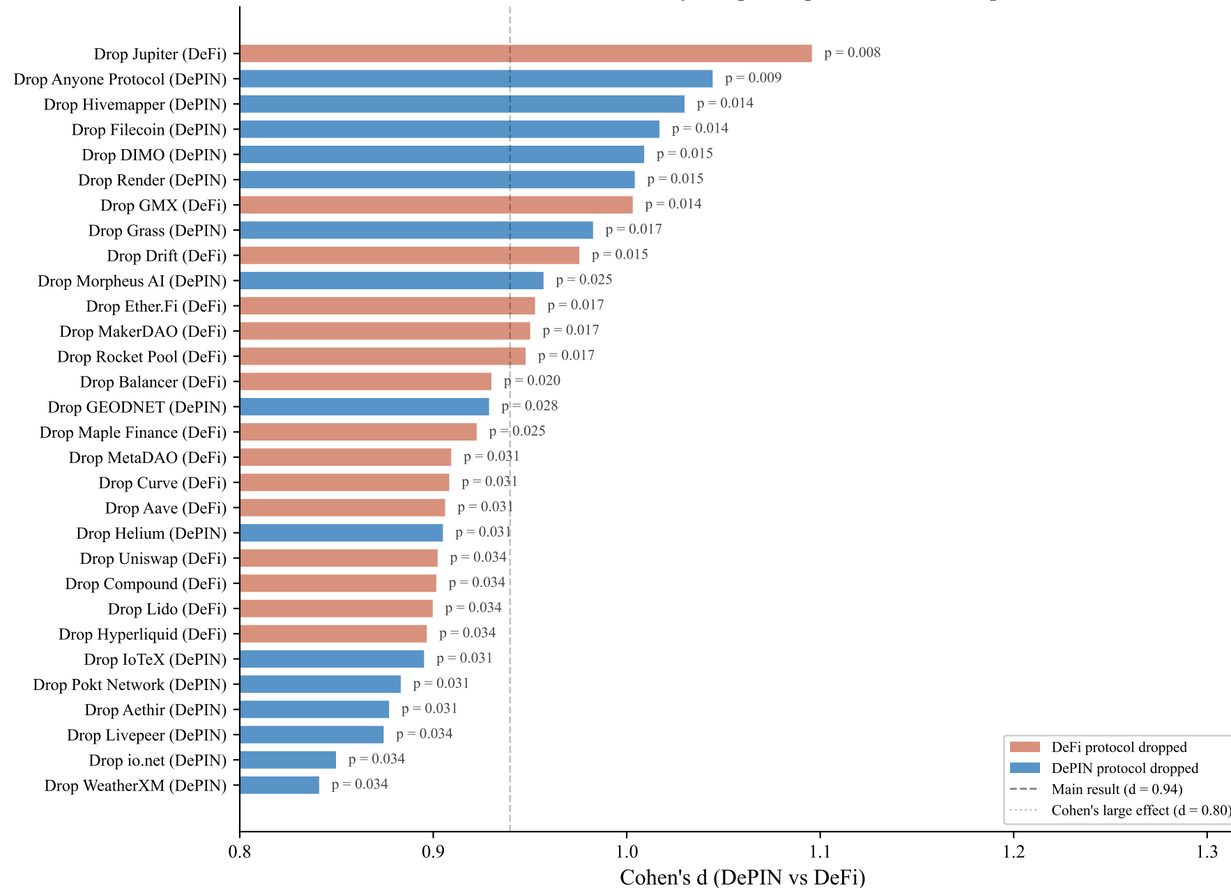
Leave-one-out sensitivity: drop each protocol and recompute
