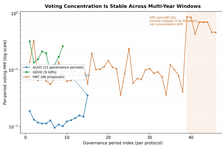
Figure 7. Per-period voting-HHI trajectories (log scale, by period index) for the three protocols with a true per-period governance series (Algorand, GEODNET, Helium; per-period values in the table above). Voting concentration is stable across multi-year windows of normal participation. The two annotated late-period excursions are artifacts rather than concentration drift: the Algorand GP15 uptick follows the post-GP14 end of rewards-eligible commitment (a 92.7 percent commitment-volume drop), and the shaded Helium post-HIP-141 region reflects a turnout collapse from the 200-to-1,024-voter range to 5-to-10 voters. Drift Protocol carries no
