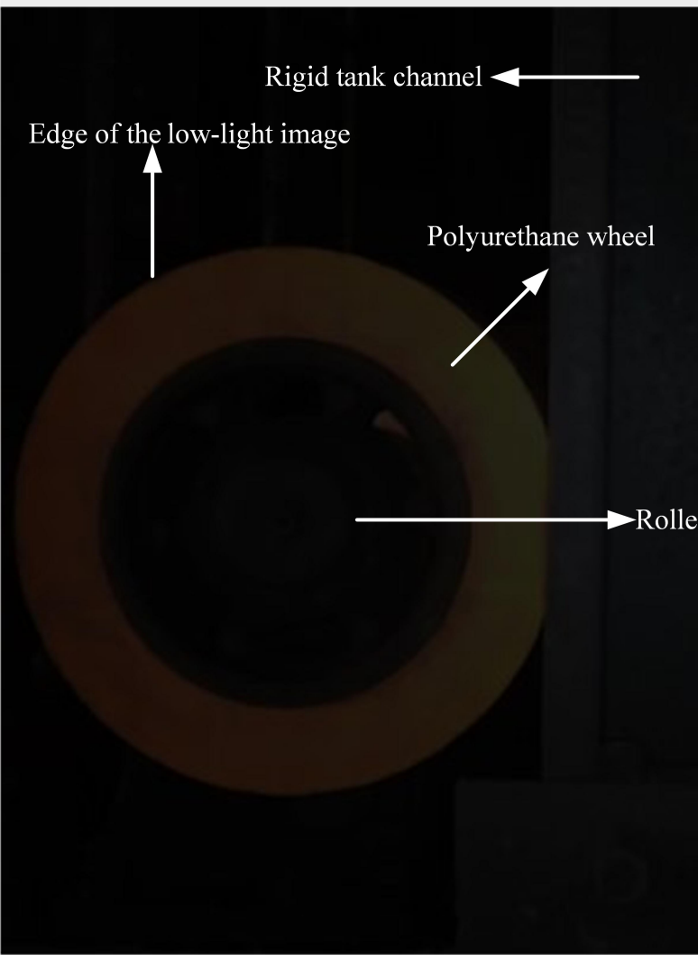
Low-light image
