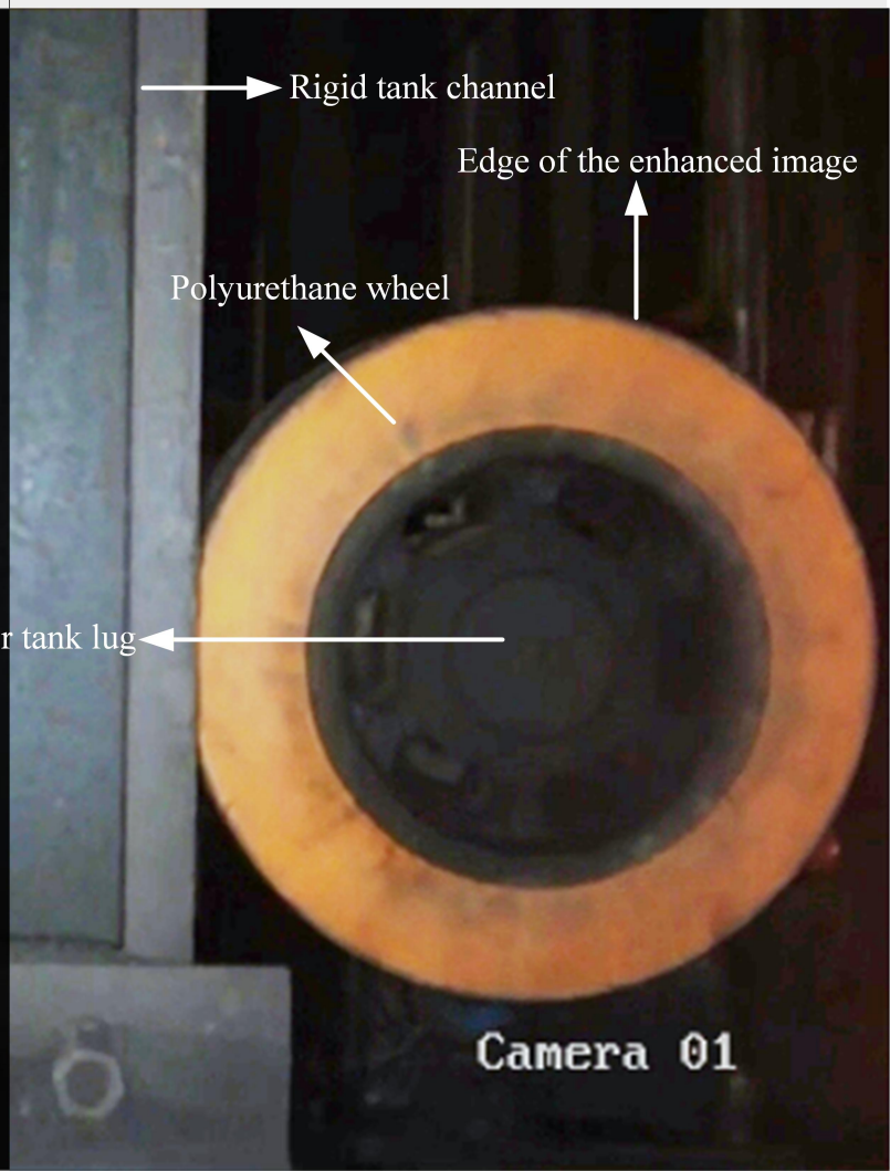
Enhanced image
