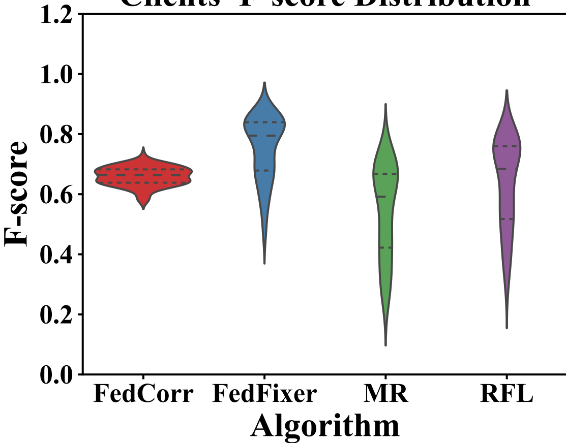
Clients' F-score Distribution
