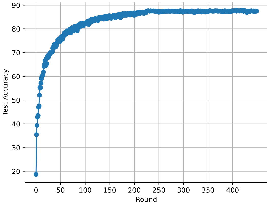
Test Accuracy vs. Round
