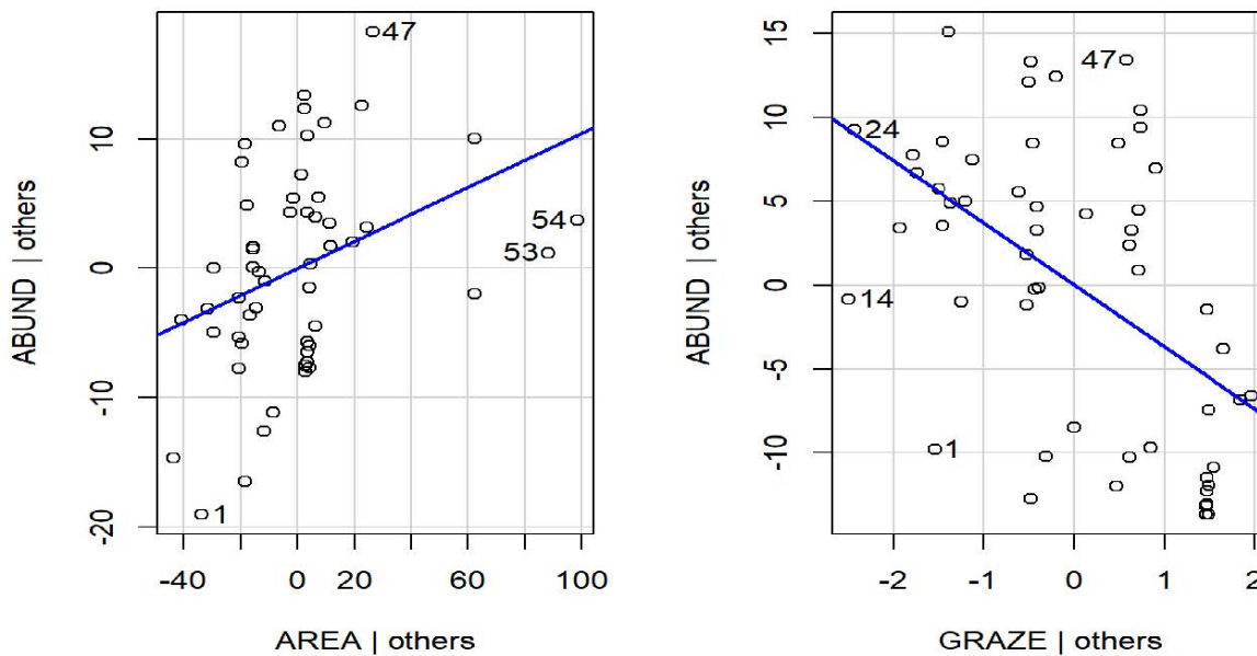
Added-Variable Plots
