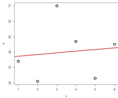
(a) R^2 = 0.012
