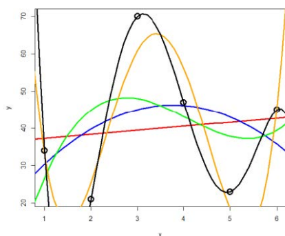
(e) R^2 = 1.000
