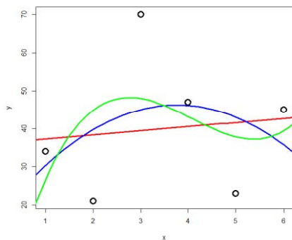
(c) R^2 = 0.170
