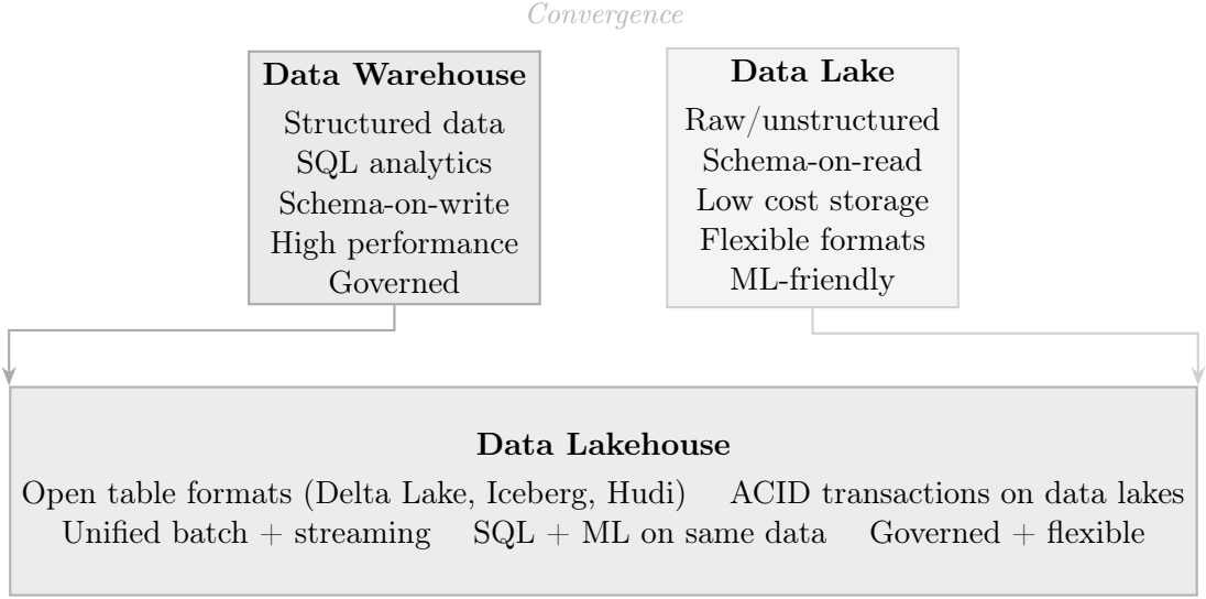
Figure 2: The data platform continuum: data warehouses and data lakes converge into the data lakehouse paradigm.
