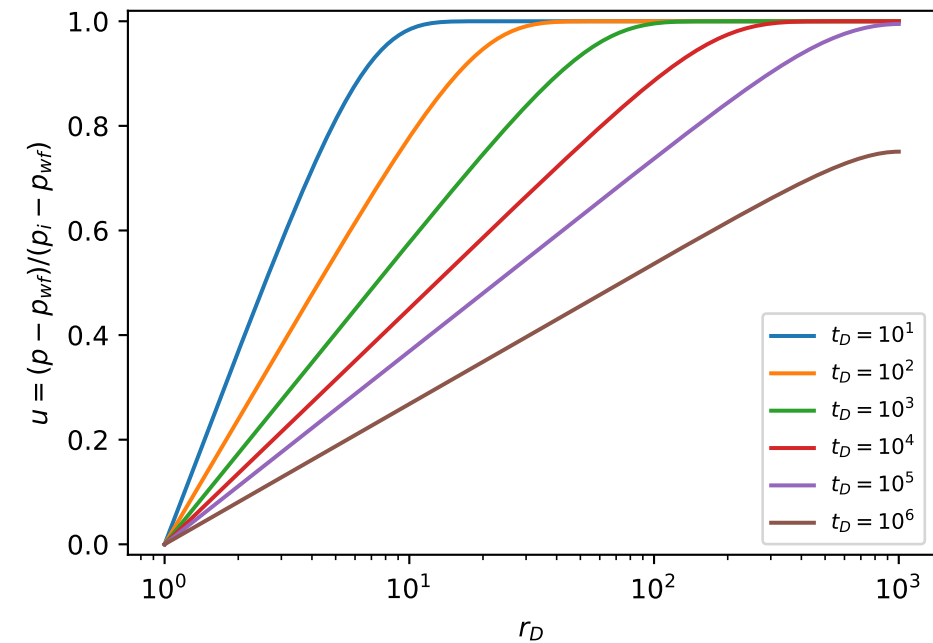
(a) pressure profiles, k_D \equiv 1
