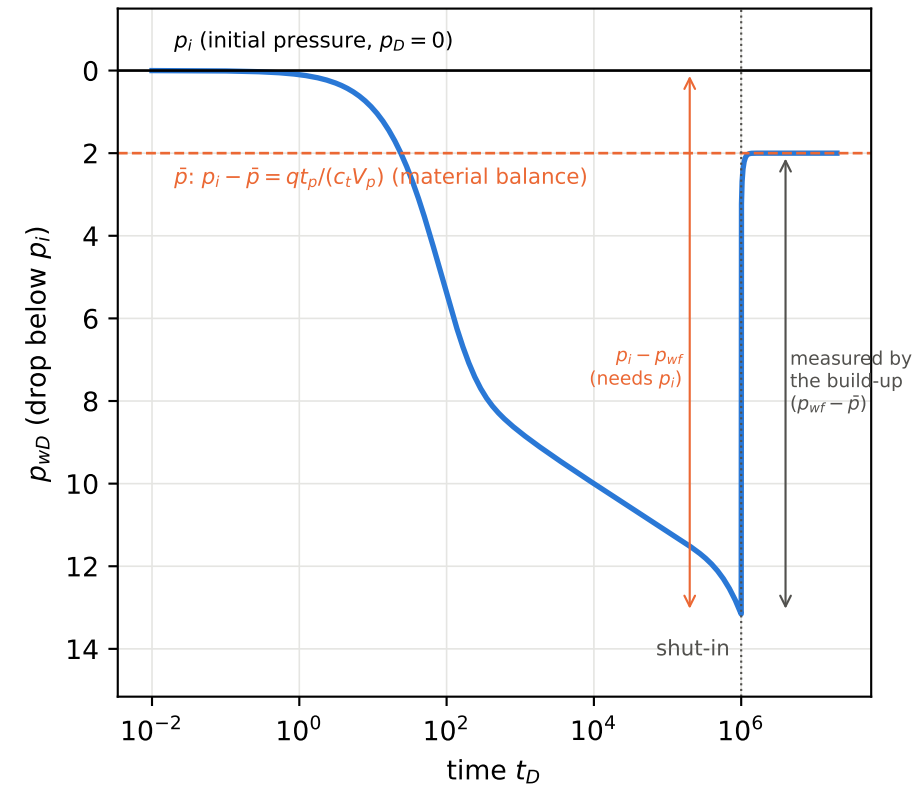
(c) history and material balance ( r_{eD}=1000 , t_p=10^6 )
