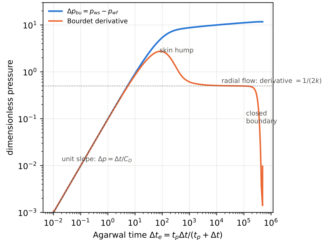
(a) log-log diagnostic plot
