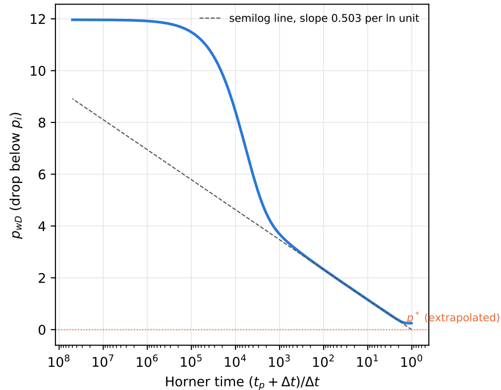
(b) Horner plot
