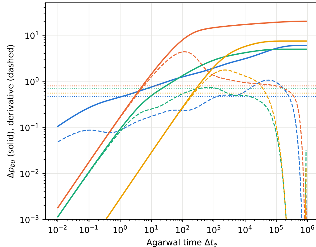
(b) log-log plot (dotted: 1/(2k_{eff}) )
