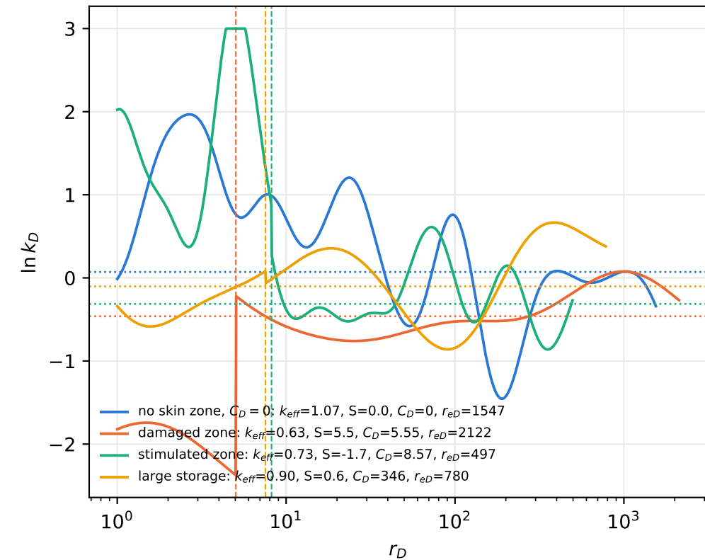
(a) permeability (dotted: \ln k_{eff} ; dashed: r_s )
