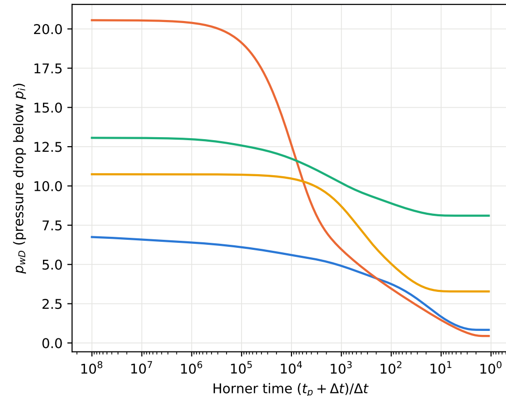
(c) Horner plot
