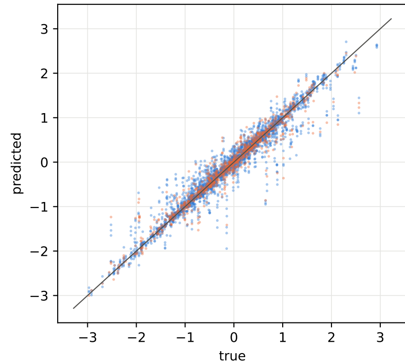
(a2) ring \ln k , r_D in [5, 10]
