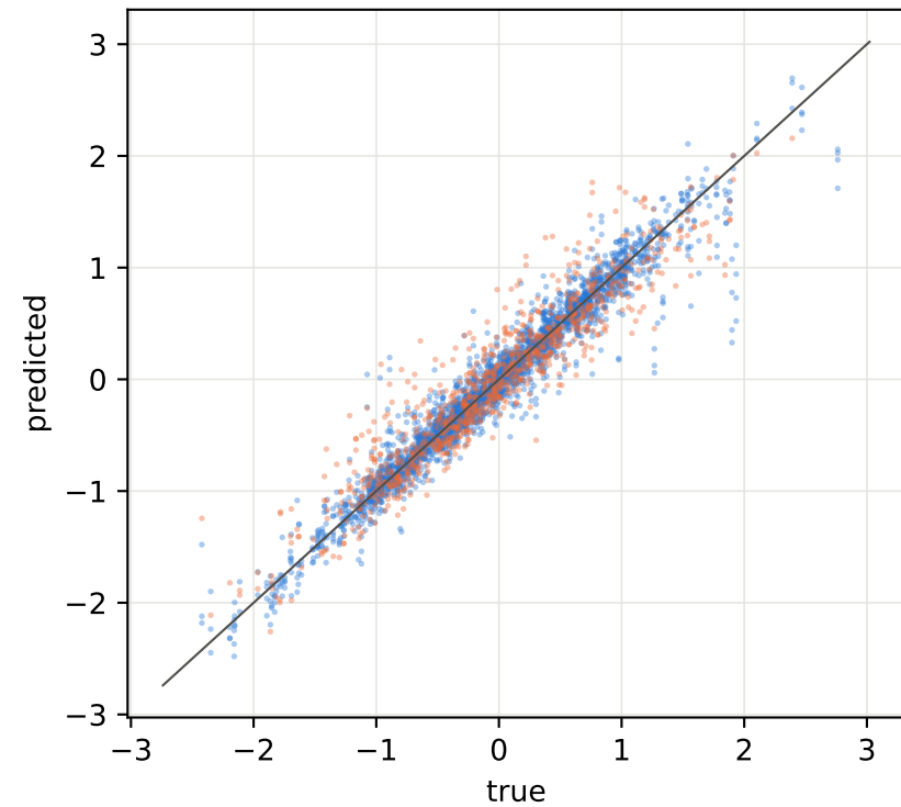
(a5) ring \ln k , r_D in [100, 300]
