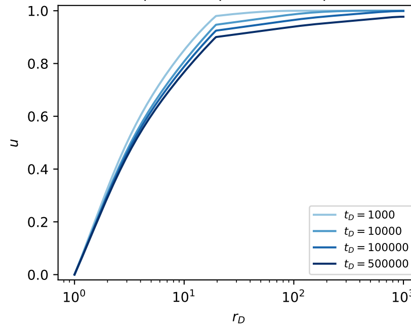
(b) pressure profiles, sample B
