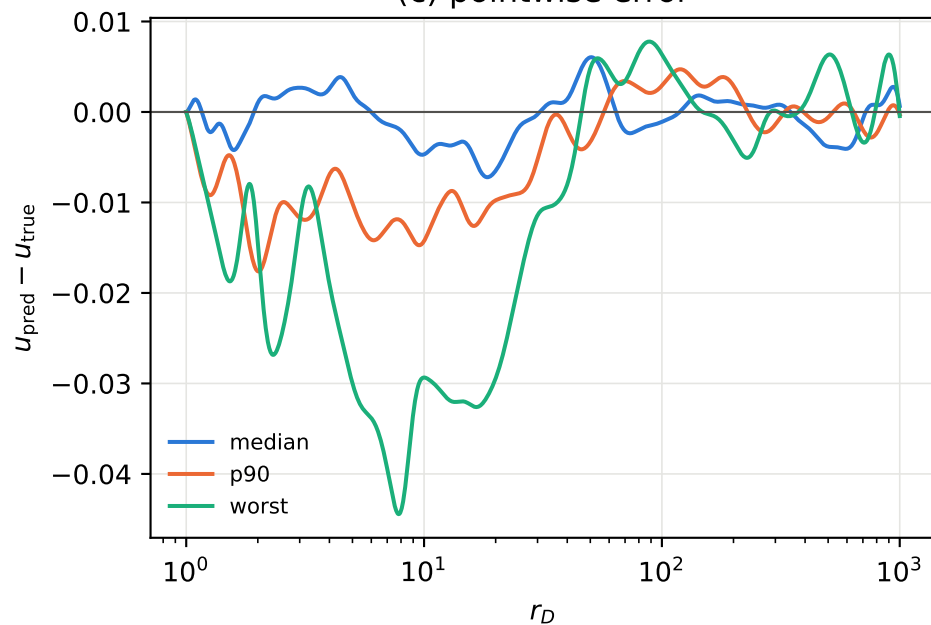
(c) pointwise error
