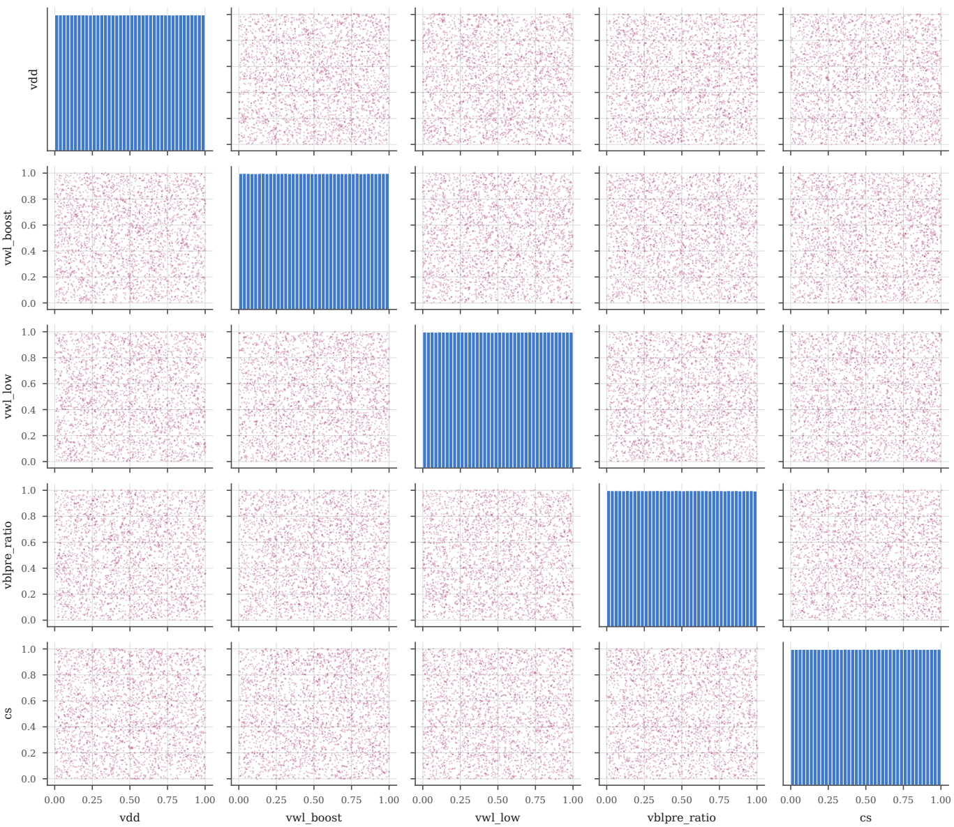
Latin-hypercube design: pairwise projections and marginals
