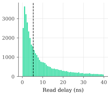
Distribution of simulated responses (dashed line: median)
