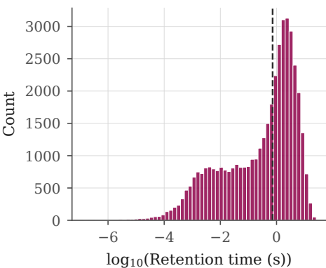
Distribution of simulated responses (dashed line: median)
