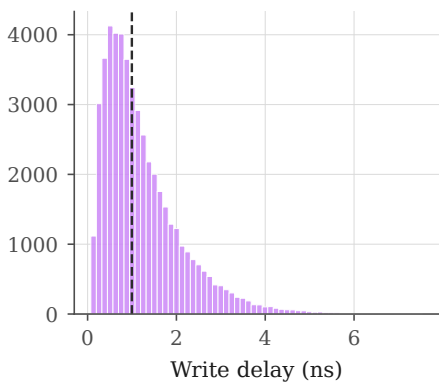
Distribution of simulated responses (dashed line: median)
