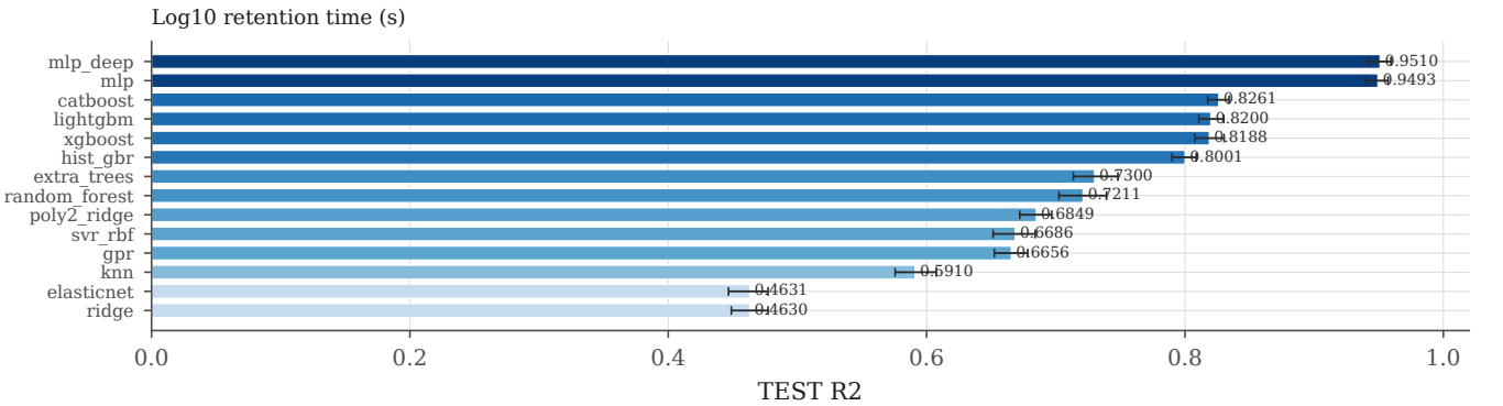
Surrogate model comparison (bars: held-out test score, whiskers: 95 % bootstrap CI)
