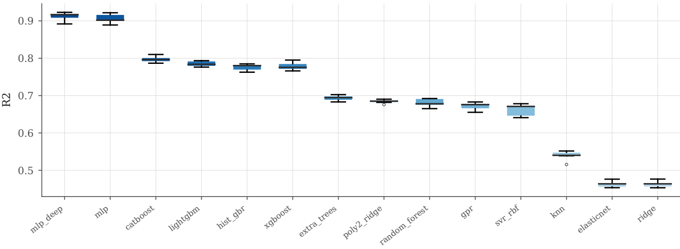
Cross-validated R2 -- Log10 retention time (s)
