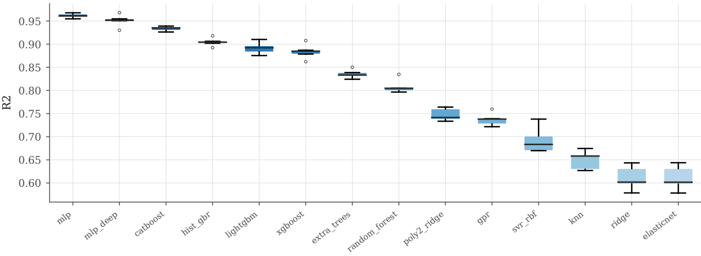
Cross-validated R2 -- Read margin (mv)
