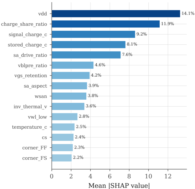
Feature importance -- Energy per access (fj)
