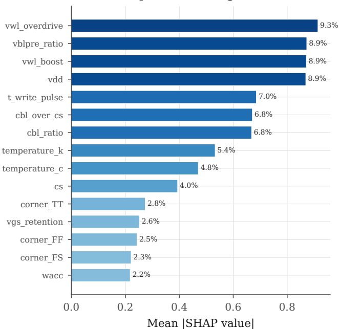
Feature importance -- Log10 retention time (s)
