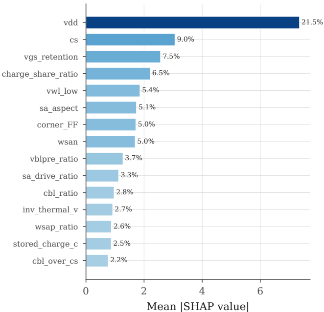
Feature importance -- Read delay (ns)
