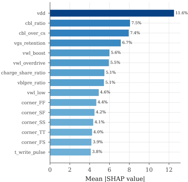
Feature importance -- Read margin (mv)
