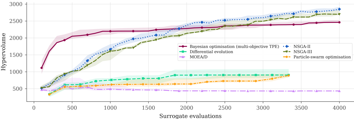
Convergence (median over independent runs, band: IQR)
