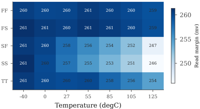
PVT corner sweep -- knee_0
