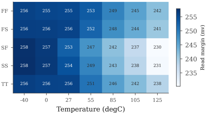
PVT corner sweep -- weighted_1
