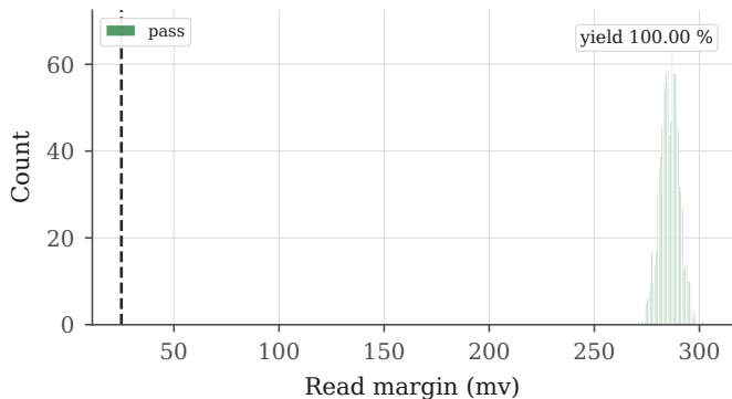
Monte-Carlo robustness -- best_read_mv_5 (dashed line: specification limit)
