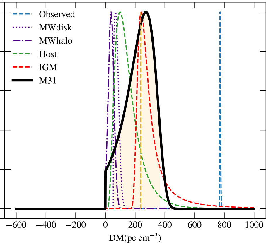
FRB 20230506C
