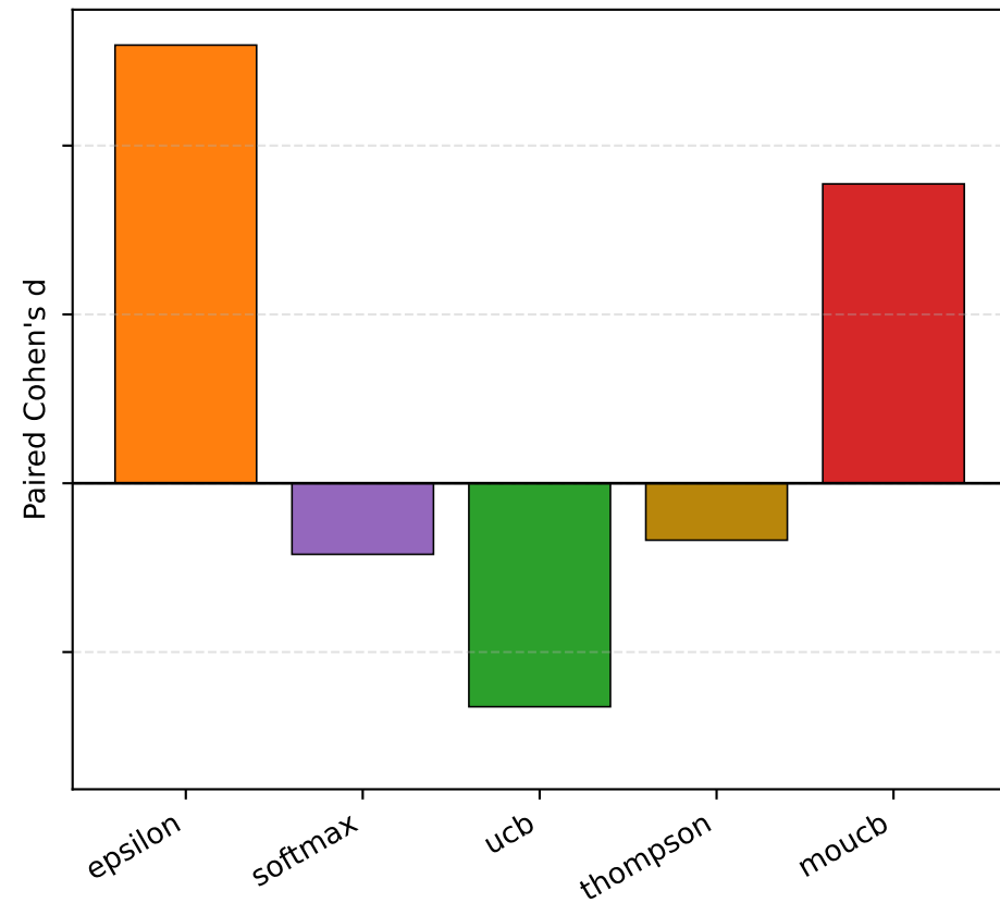
tests
