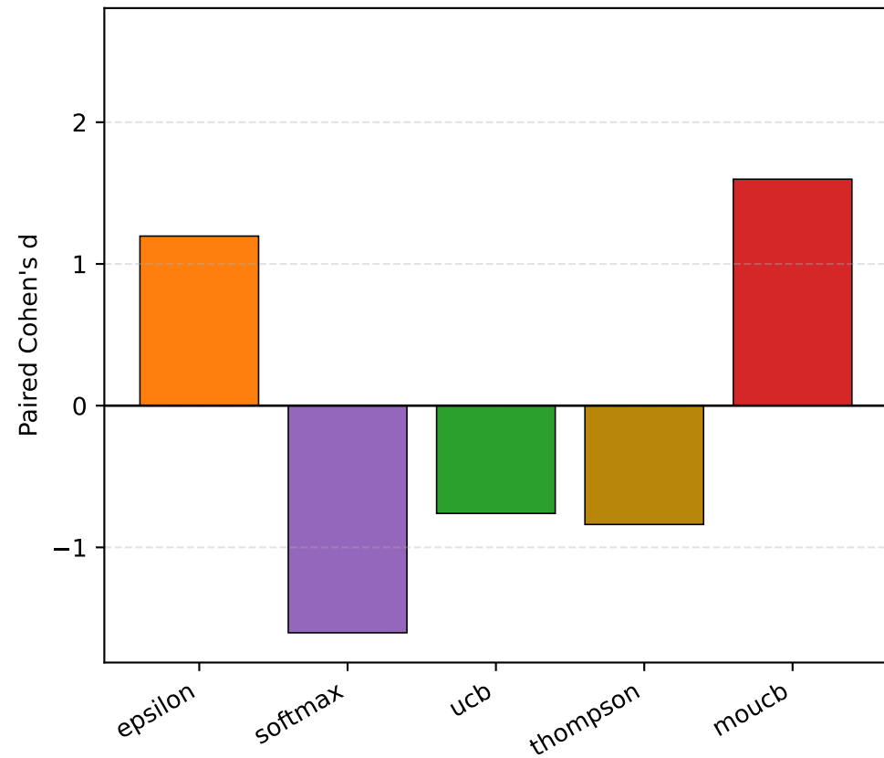
code
