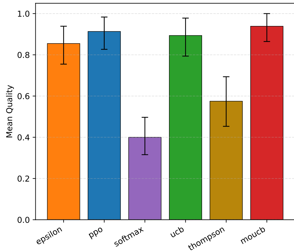
code
