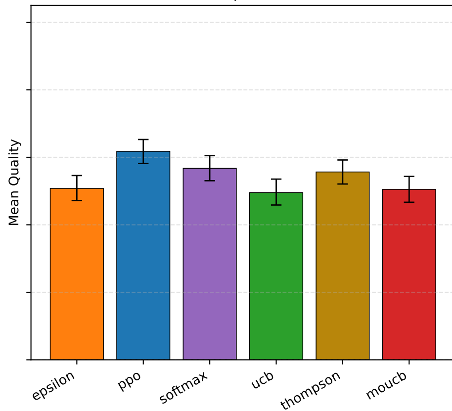
explain
