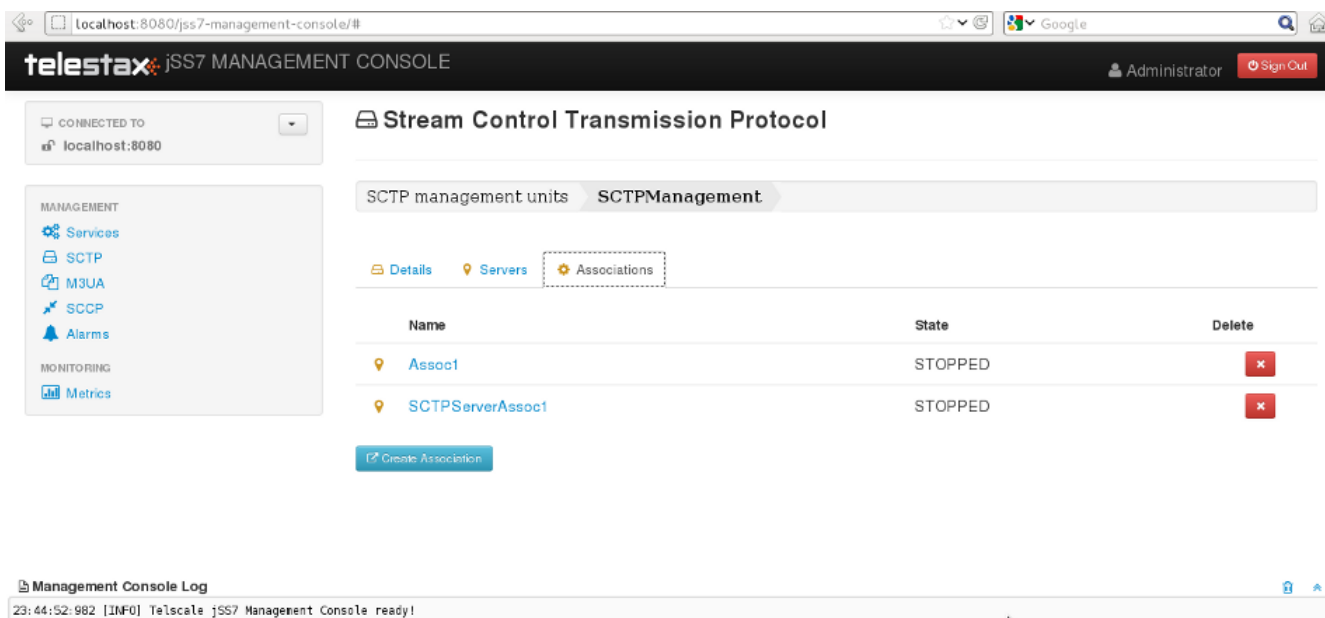
Figure 17. GUI - SCTP Management - Associations
