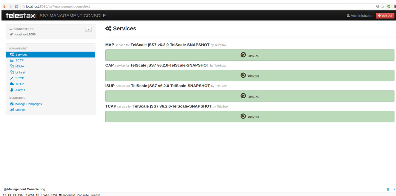
Figure 5. GUI - Services
