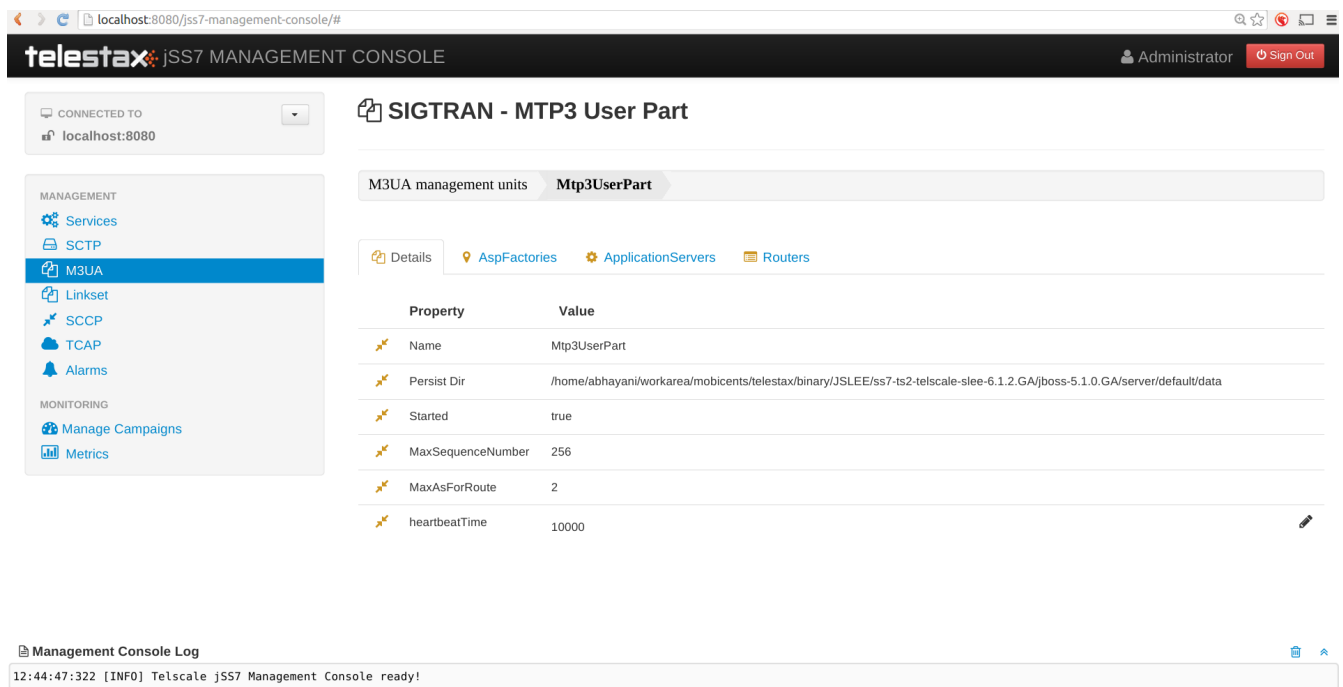
Figure 18. GUI - M3UA Management
