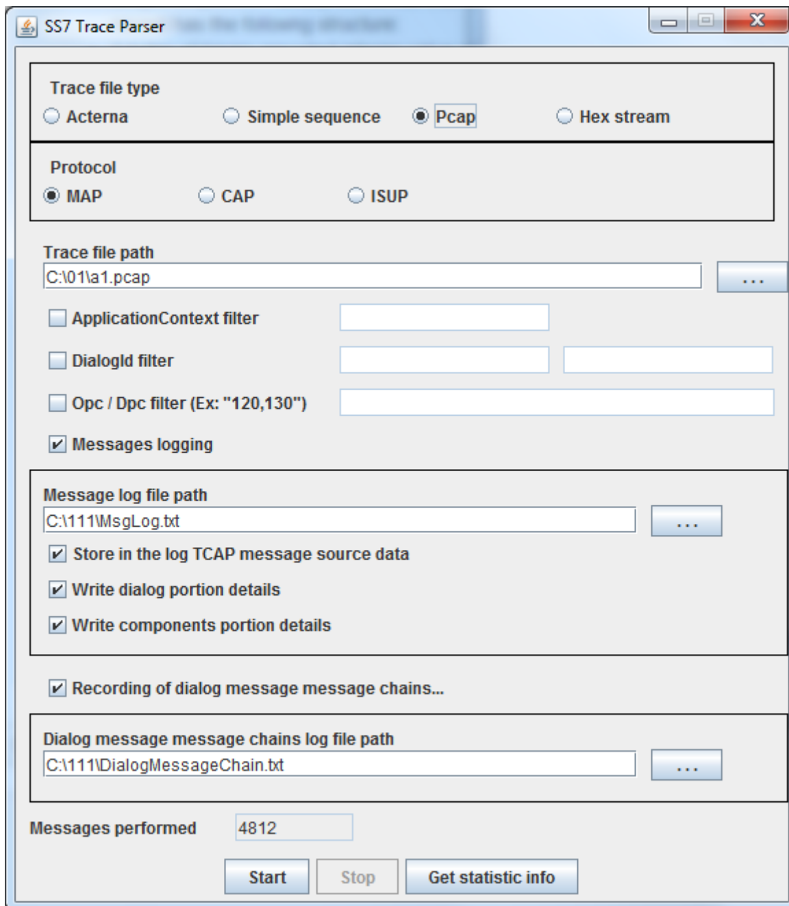
Figure 45. Running Trace Parser
