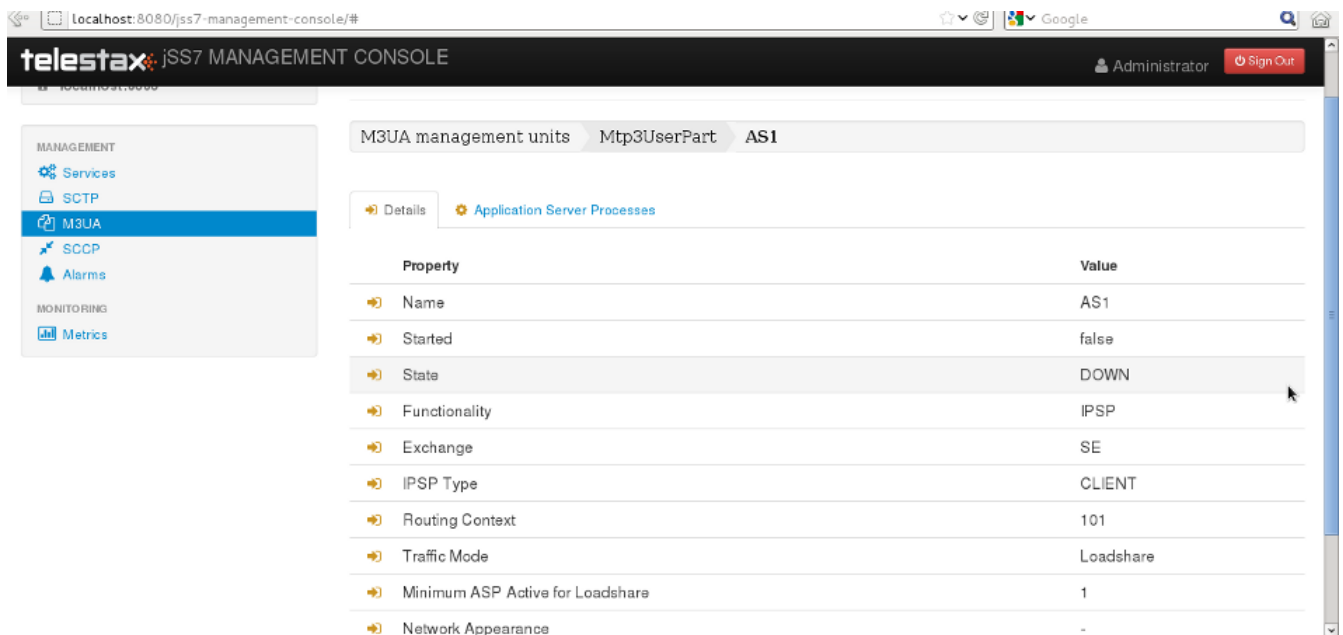
Figure 22. GUI - M3UA Management - AS Details
