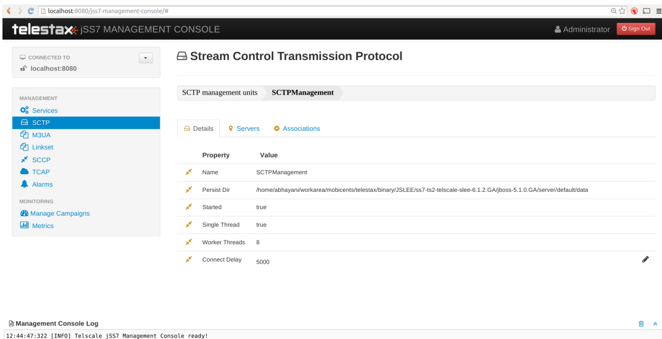
Figure 13. GUI - SCTP Management
