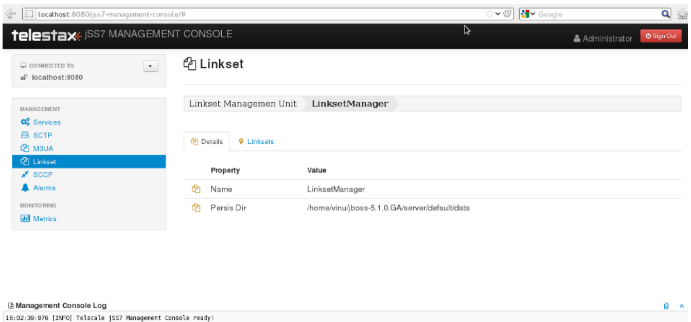
Figure 12. GUI - Linkset Management
