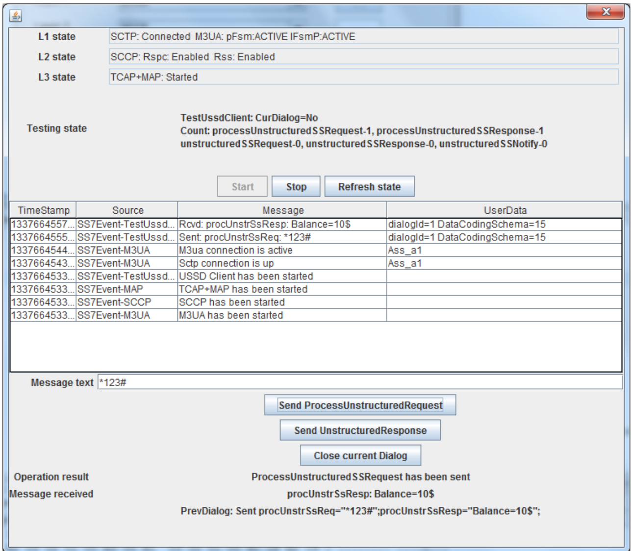
Figure 8. Example Simulator testing form
