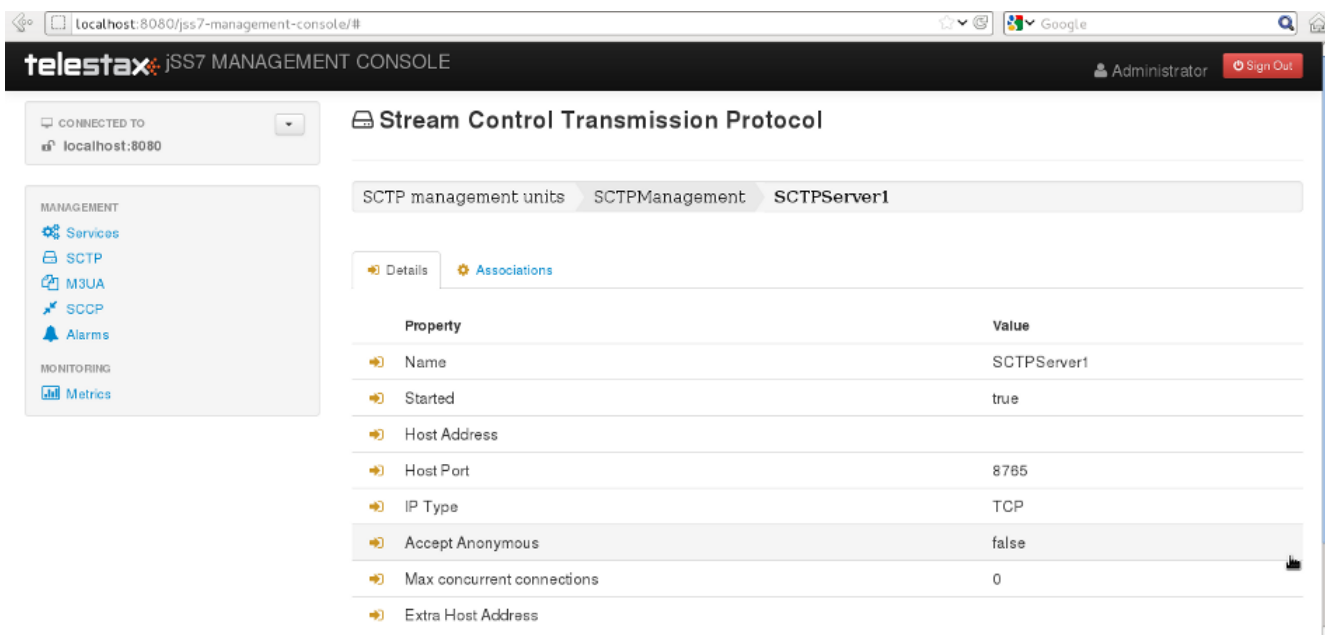
Figure 15. GUI - SCTP Management - Server Details
