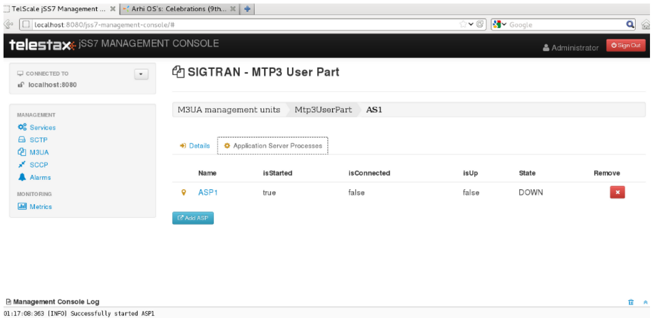
Figure 23. GUI - M3UA Management - Assign ASP to an AS
