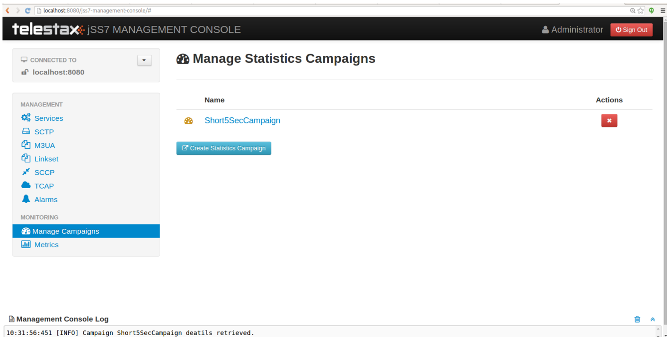
Figure 27. GUI - Campaigns
