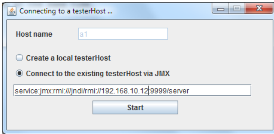
Figure 9. Launching Simulator GUI for a remote mode
