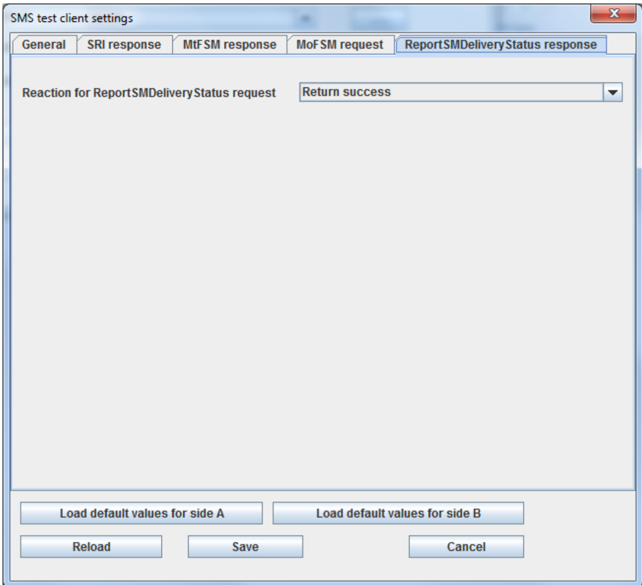
Figure 41. SMS client settings form
