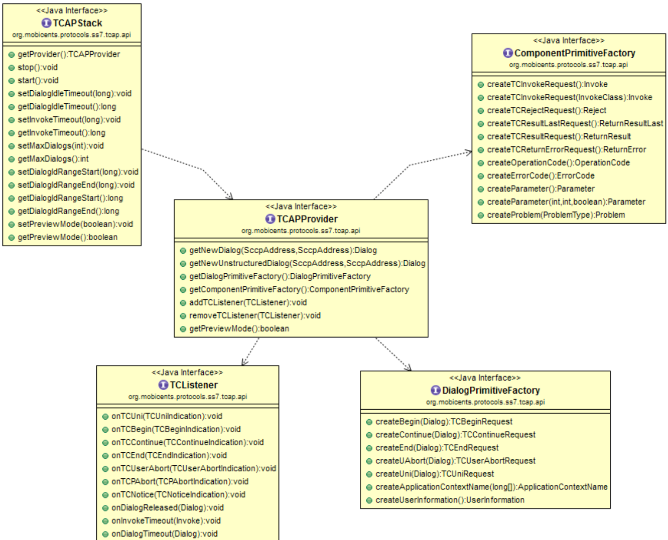
Figure 36. Restcomm jSS7 Stack TCAP Class Diagram
