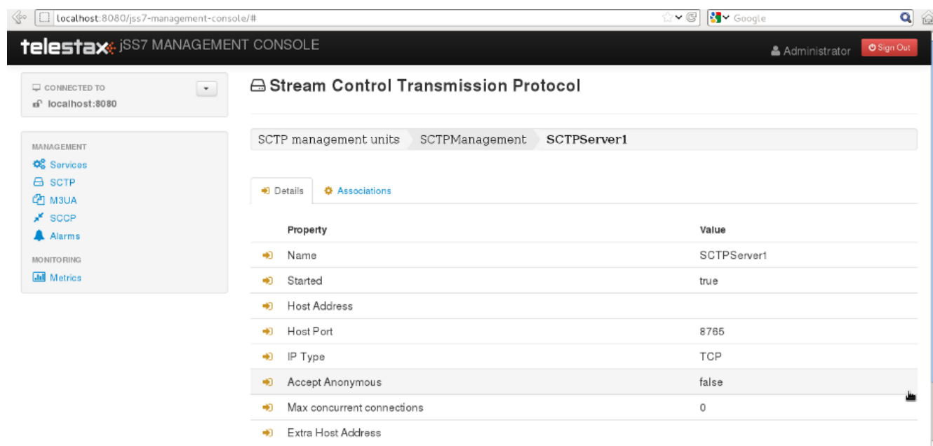
Figure 16. GUI - SCTP Management - Server Create
