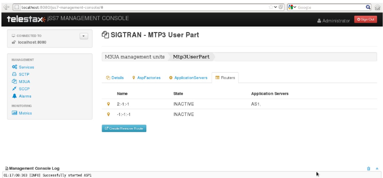
Figure 24. GUI - M3UA Management - Route
