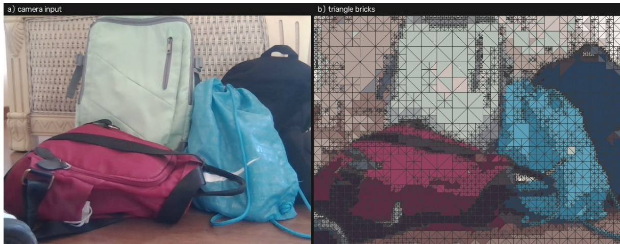
Figure 14. A real camera frame beside its triangle-brick render ( K = 16 , 9,990-brick quality preset), shown at the 640 \times 480 the loop runs at. Input and render appear together because a mosaic judged without its input says nothing about fidelity. This scene is the clearest single demonstration of the two adaptive decisions working together: the partitioner puts its smallest cells on the bag seams, zips and handles while the flat wall behind stays in large coarse cells, and the 16-colour Lab palette keeps the sage-green, teal and maroon cases apart instead of collapsing them into one lukewarm average. The two panes are not the same brightness, though: the render is more vivid than the input, because a brick mean is assigned the nearest palette entry and the nearest entry to a saturated colour is a more saturated one. The consistent colour artefact I discuss below is on the portraits, not here.
