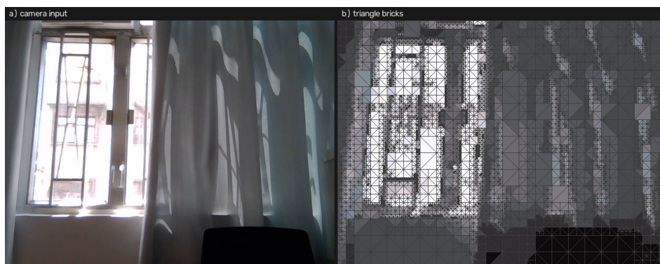
Figure 19. Sheer curtain against a window. Almost all of the structure in this frame is in the shading rather than the hue: the folds barely change colour, so what carries them is brick density — the fold boundaries get rows of small cells and the smooth panels between them get large ones. The window frame stays visible as a hard geometric boundary. It is the clearest evidence in the set that the tessellation is responding to local contrast, not to colour boundaries.
