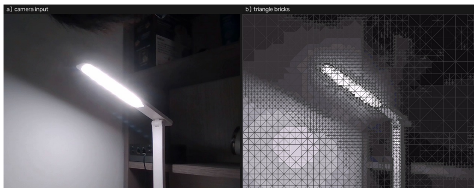
Figure 18. Desk lamp in a dim room, the extreme dynamic-range case. The light source is clipped in the input, and the render keeps it legible rather than bleeding it across the wall, because the saturated region attracts the finest cells. The surrounding shadows are the weak part: they are posterised into large flat cells, and the dark side of the frame picks up a visible cool cast from the palette's dark end. This is the case that motivated capturing with -lock-ae — an unlocked camera would normalise the exposure differently frame to frame and the mosaic would drift with it, so the flag is what makes a fixed-palette assumption safe here.
