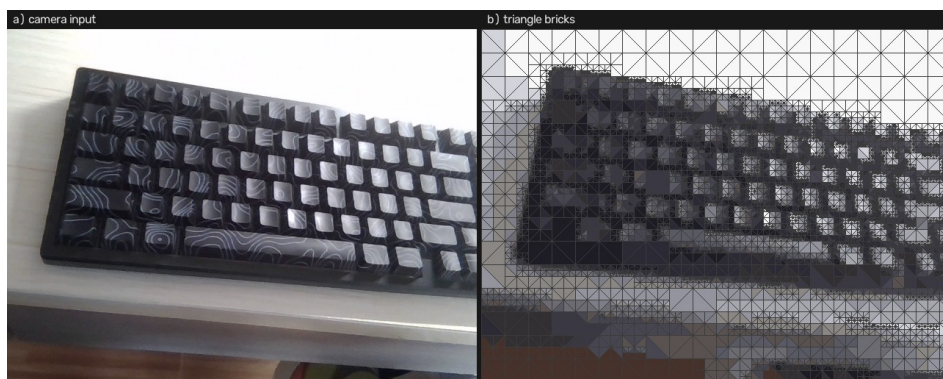
Figure 17. Mechanical keyboard. The densest high-frequency texture in the set. Two different things are being asked of the pipeline at once: the partitioner has to be small enough to resolve individual keycaps, and the palette has to keep adjacent keys from collapsing into one another. The key field is covered in the smallest cells in the whole sweep, while the desk below it — a much larger, much flatter region — stays in large cells. The keys themselves carry a marbled pattern, and the render reproduces it as mottling rather than resolving it, which is an honest limit of a 16-colour palette on a texture that varies in hue at a scale smaller than one brick.
