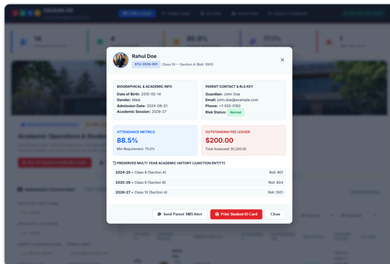
Figure 7.2: Interactive Student 360° Profile Modal displaying high-resolution student avatar portrait, biographical details, guardian RLS key, attendance compliance (88.5%), fee ledger ($200.00), and preserved multi-year junction progression history.
