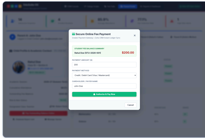
Figure 3.2: Self-Service Parent Online Fee Payment Gateway with instant credit/debit/UPI checkout and automated Zoho CRM financial ledger synchronization.
