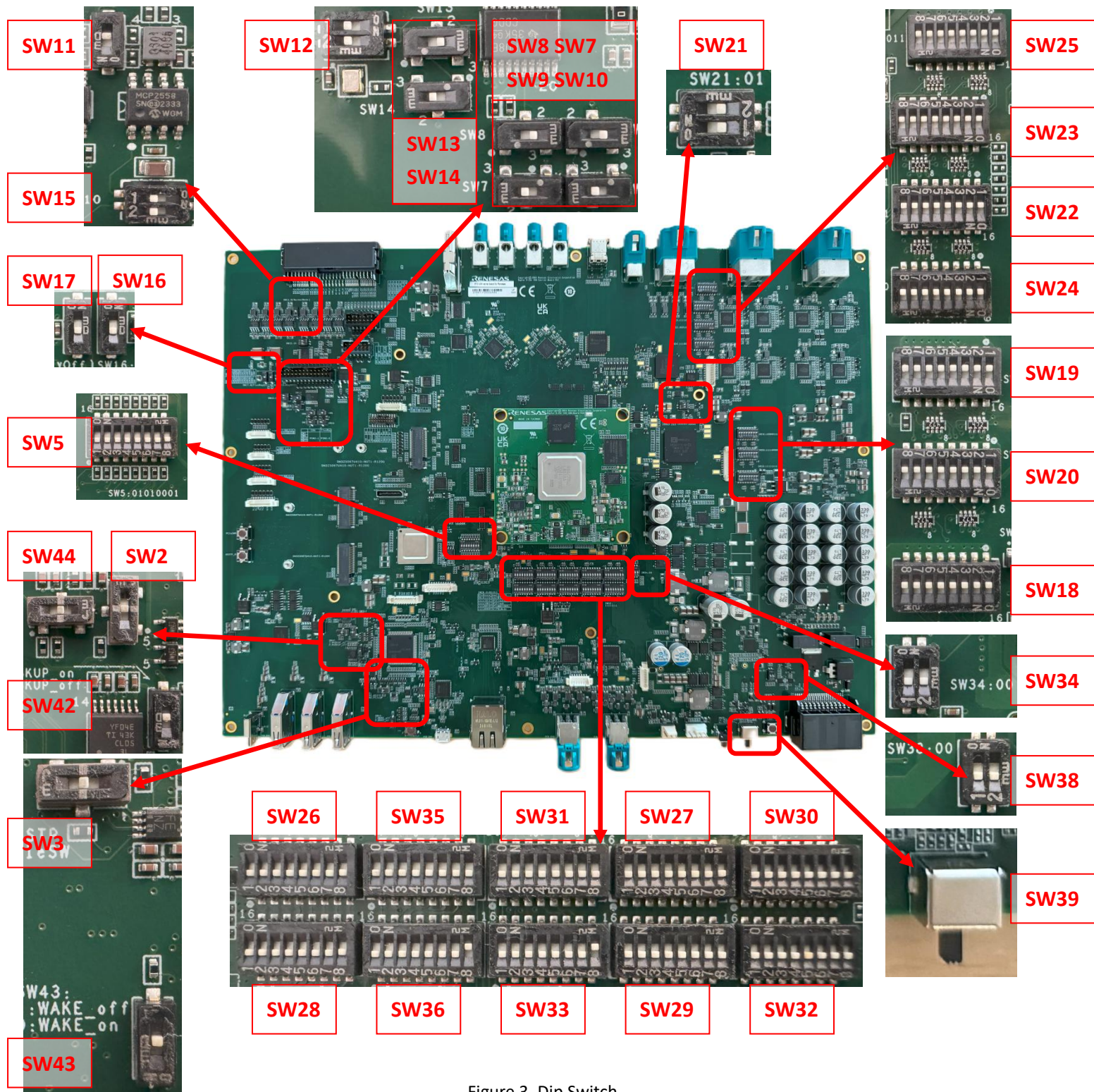
Figure 3. Dip Switch
