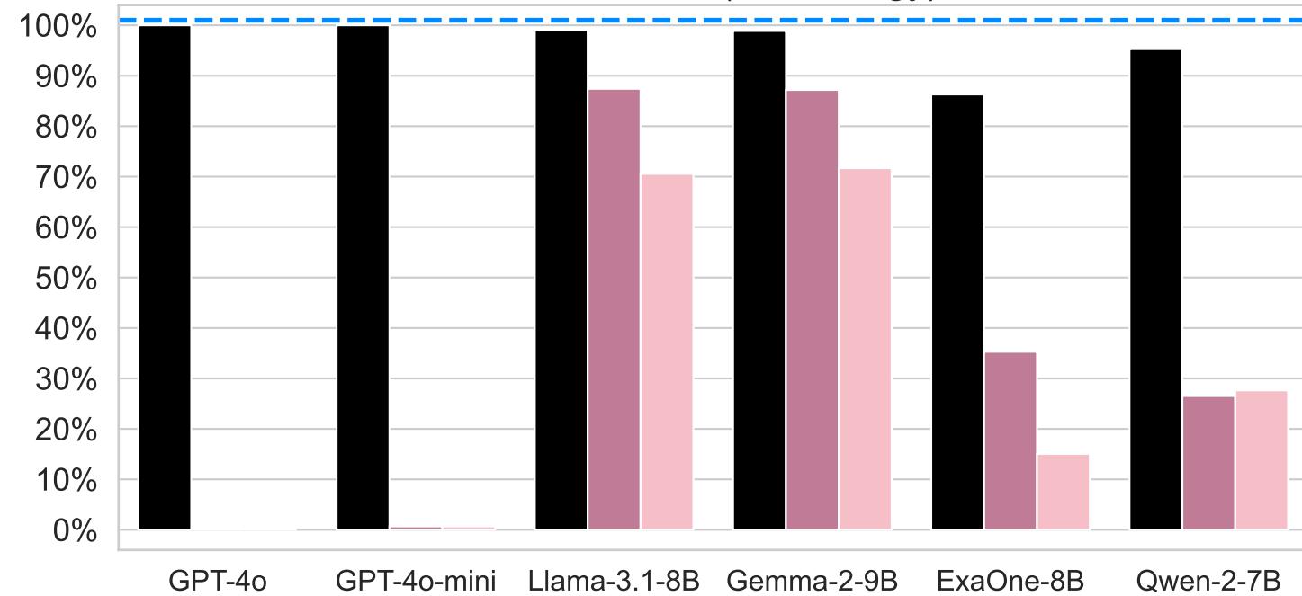
True Positive (Deontology)
