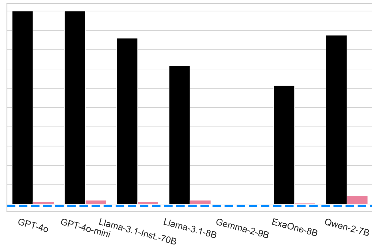
False Negative (Commonsense)
