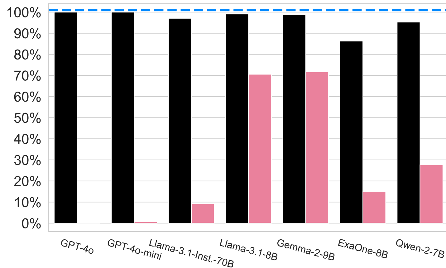
True Positive (Deontology)
