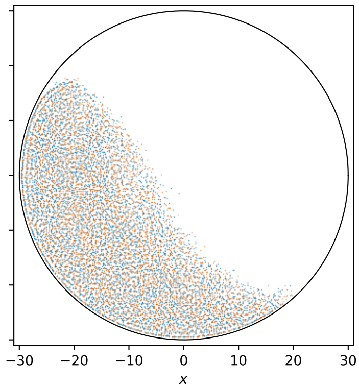
Final stationary snapshot t = 1720.721
