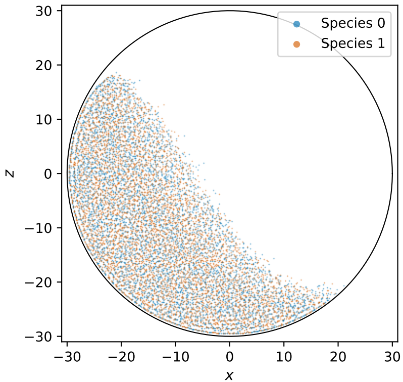
First stationary snapshot t = 1378.133
