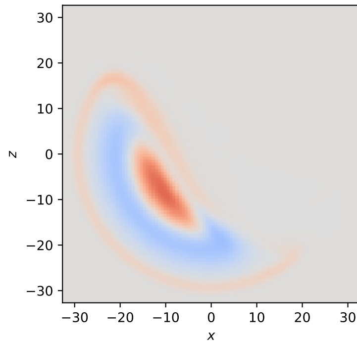
Centred POD mode 5
