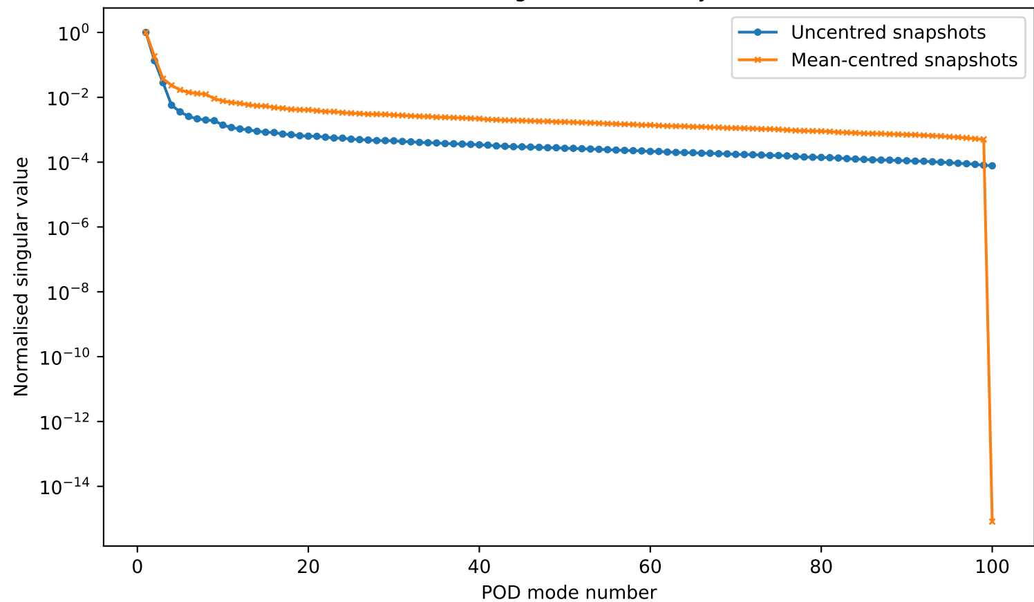
POD singular-value decay
