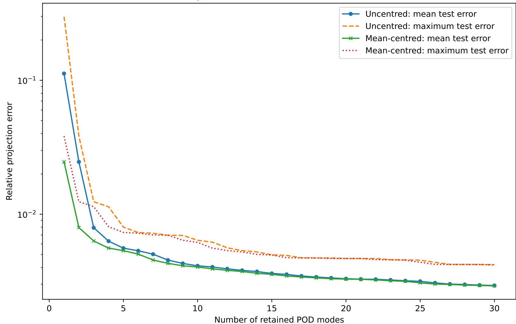
POD representation errors on unseen test fields
