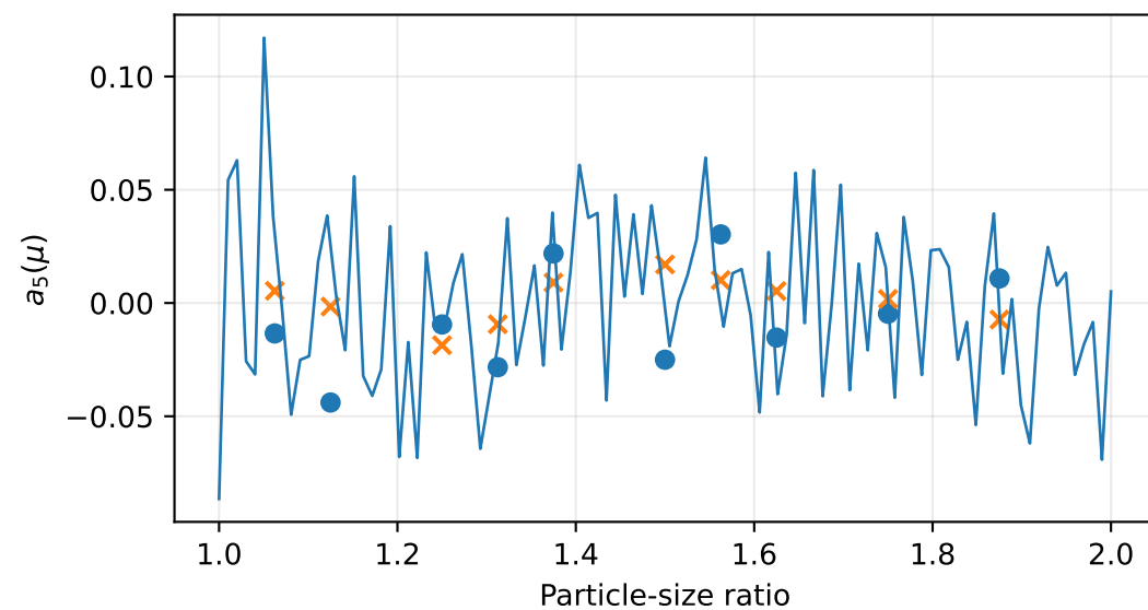
POD coefficient 5
