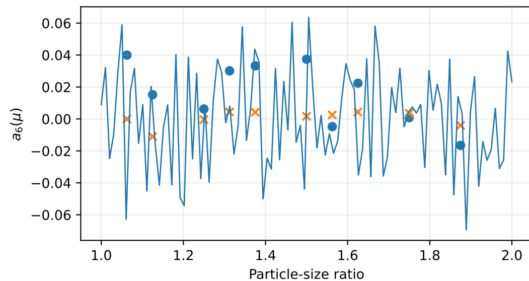
POD coefficient 6
